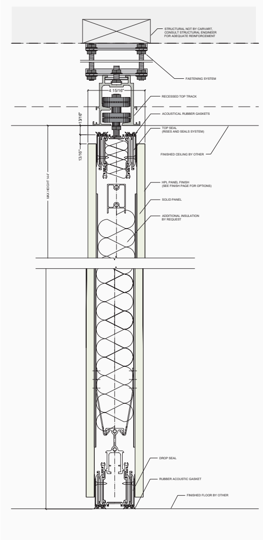
TYPICAL VERTICAL SECTION
