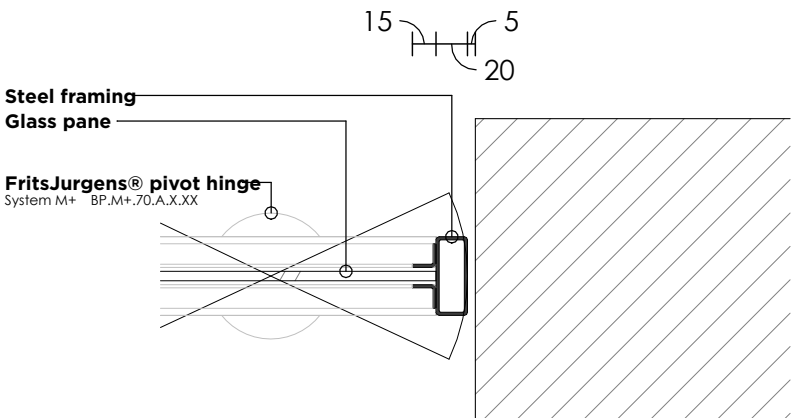
Detail 3 1:5
