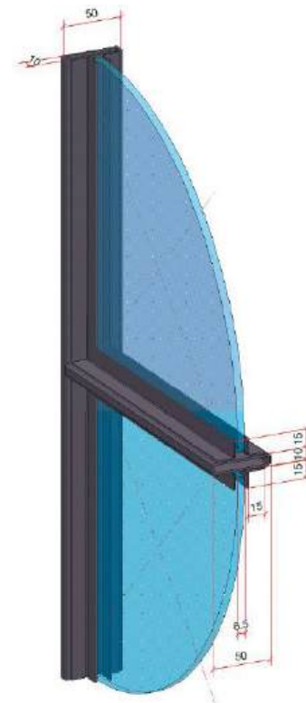
PROFILE DETAIL
