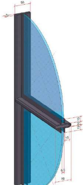
PROFILE DETAIL
