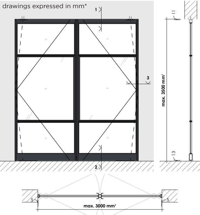
SECTIONS DETAILS
