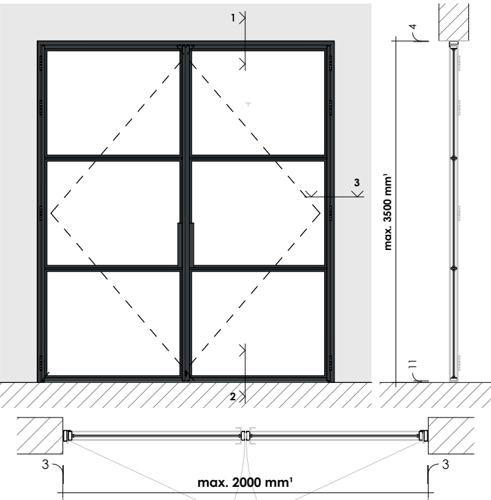
SECTIONS DETAILS
