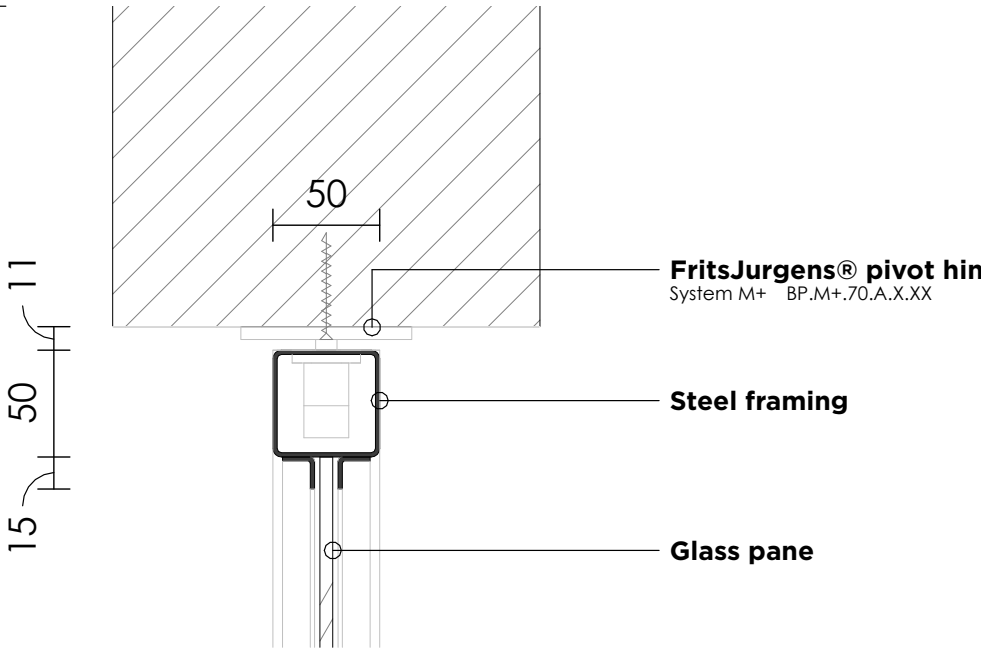
Detail 1 1:5
