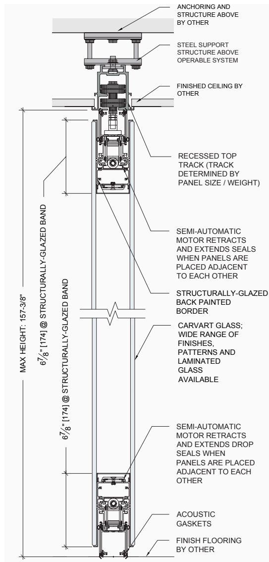
VERTICAL SECTION
