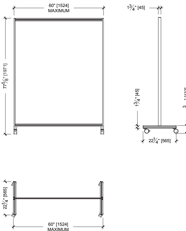
TYPICAL DETAILS
