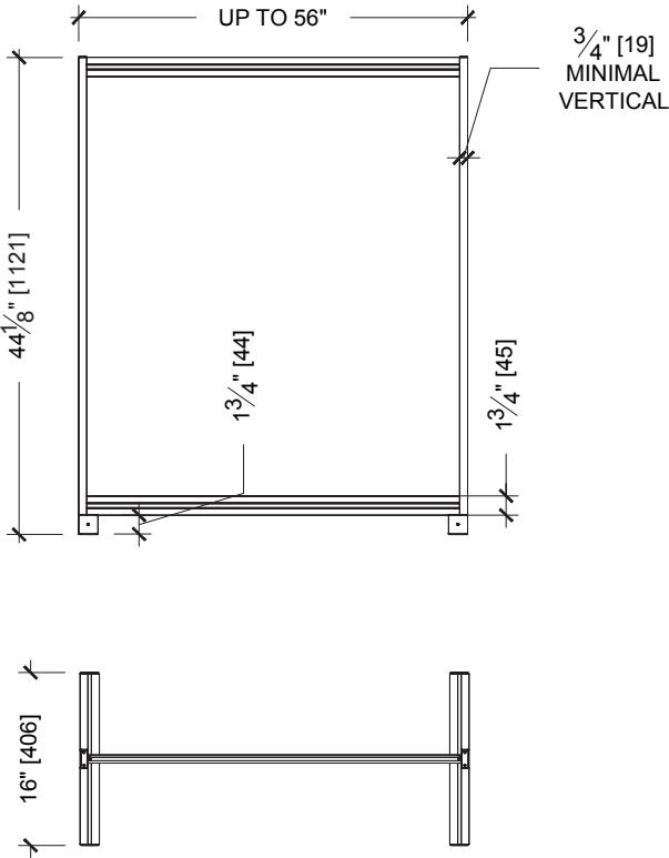
TYPICAL DETAILS
