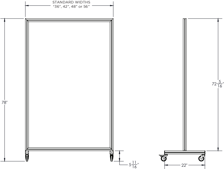
TYPICAL DETAILS
