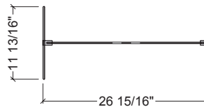
TYPICAL DETAILS
