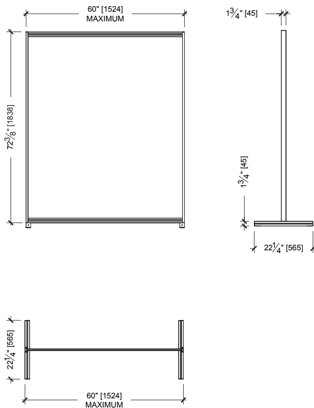
TYPICAL DETAILS
