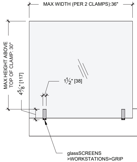
TYPICAL ELEVATION
