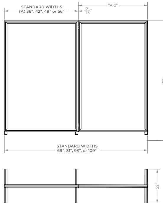
TYPICAL DETAILS
