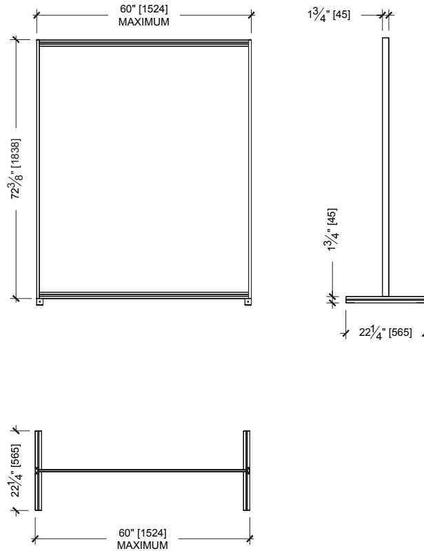
TYPICAL DETAILS
