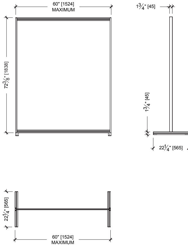
TYPICAL DETAILS
